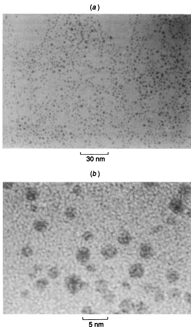
Fig. 1 TEM pictures of the thiol derivatised gold nanoparticles at (a) low and (b) high magnification
